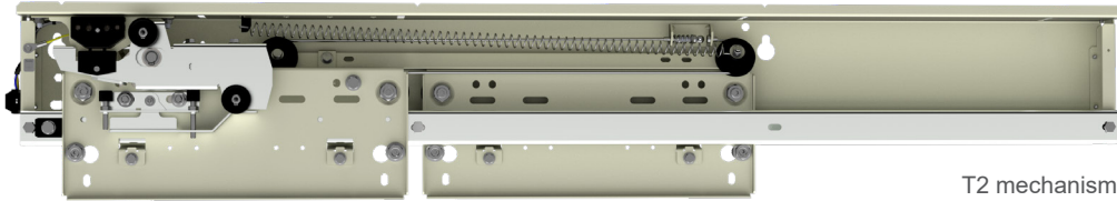
T2 mechanism
